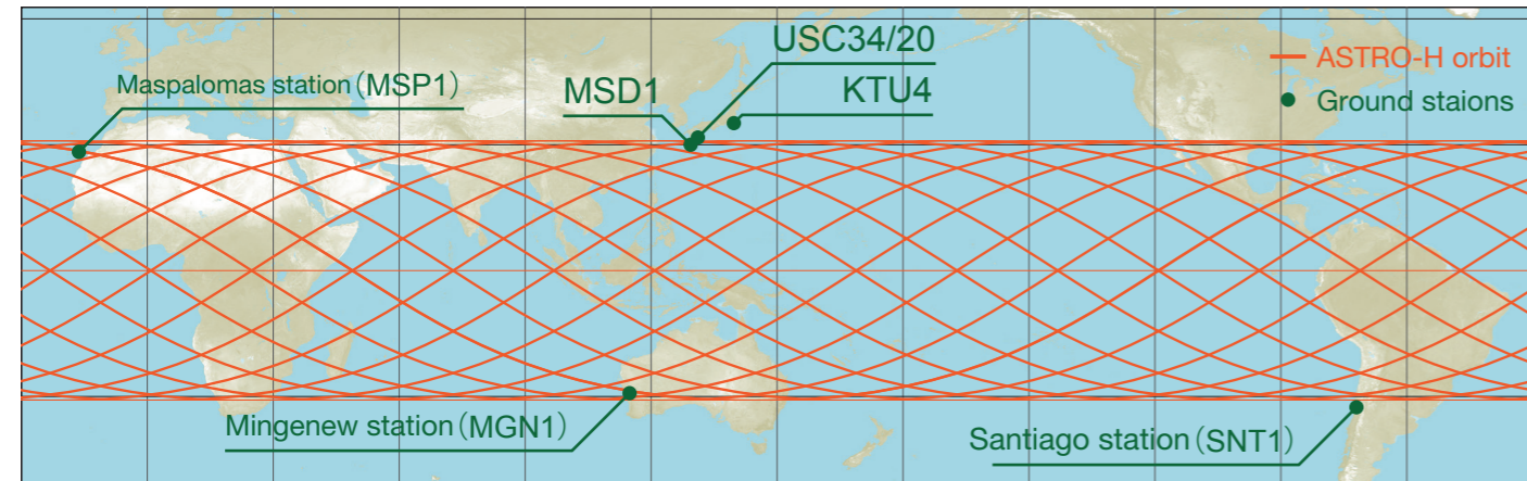
Figure 3.11: Location of the ASTRO-H ground stations with ASTRO-H orbits. ASTRO-H orbits around the earth every 96 mins. The spacecraft receives sunlight for 2/3 of a day and it is in shade for 1/3 of the day, while it goes around 15 times a day. ASTRO-H will be visible from Japan 5 times out of the 15. It will be in communication for about 10 min during each pass. During that time, commands will be sent and data will be downloaded to the ground.
