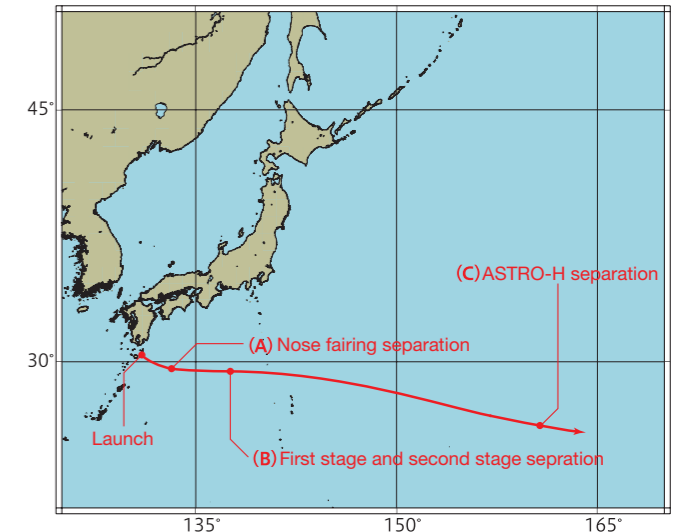
Figure 3.6: Rocket trajectory until the ASTRO-H separation with major events.
