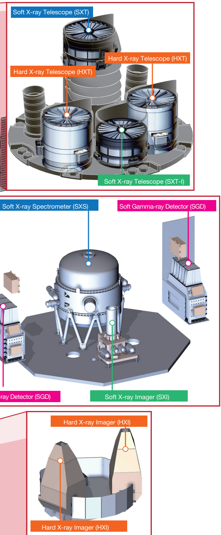
Figure 3.2: ASTRO-H Instruments
