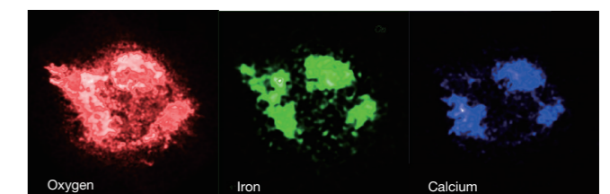
Figure 1.7: Distribution of various elements in supernova remnant Cassiopeia A. (NASA/GSFC/U.Hwang et al.)
