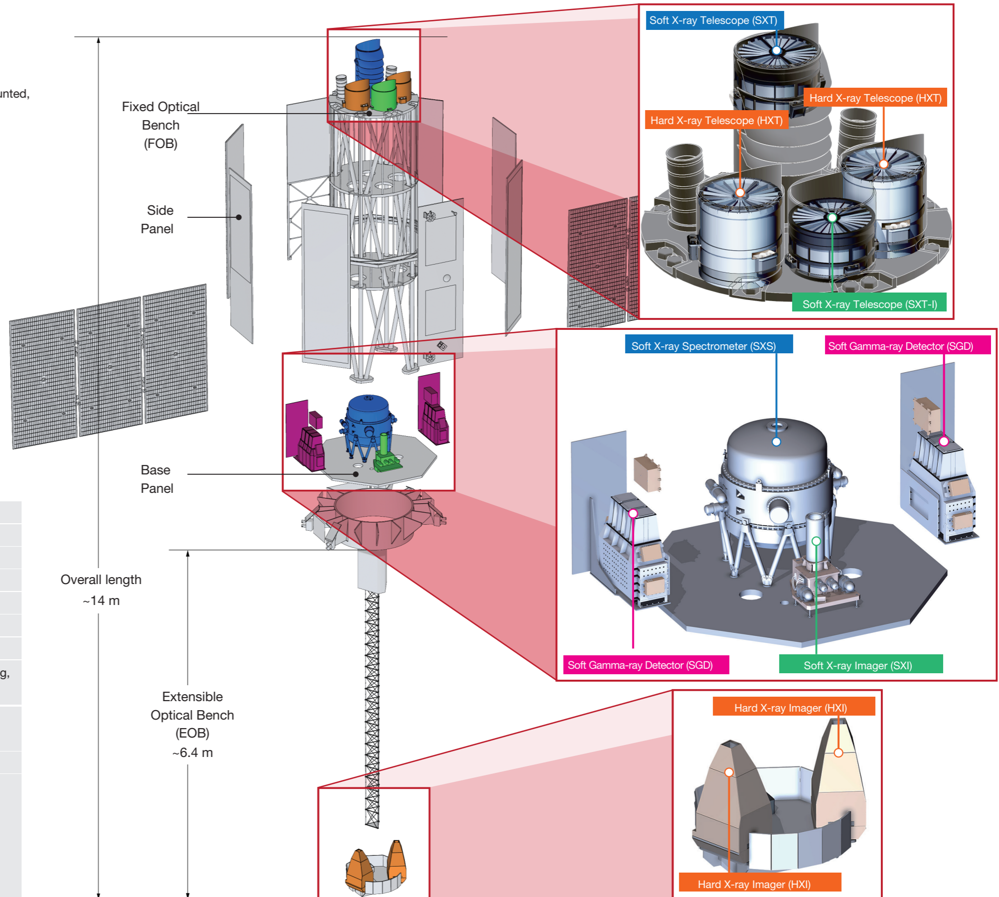
Figure 3.1: ASTRO-H architecture
