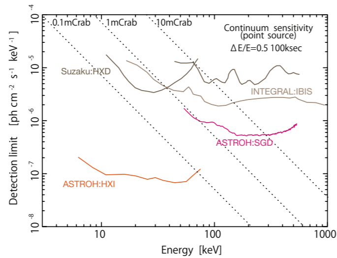
Figure 3.4: Energy band and limiting sensitivity of ASTRO-H hard X-ray/soft Gamma-ray instruments. Suzaku and INTEGRAL (ESA) are also shown for comparison. HXI and SGD have 100 and 10 times greater sensitivity over Suzaku, respectively.
