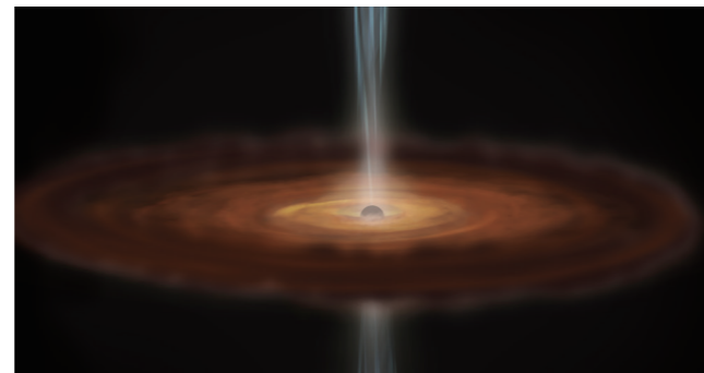
Figure 1.2: Illustration of a black hole. Not only are X-rays emitted by matter accreted by black holes, they are also emitted when a fraction of the accreted matter is beamed out.
