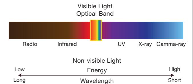
Figure 1.4: Electromagnetic spectrum in energy and wavelength
