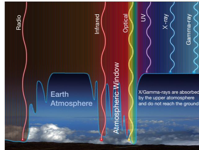
Figure 1.8: Atmospheric transmission and lights with various wavelength. Atmospheric window is a wavelength band where light is less absorbed by the atmosphere and can reach the ground.
