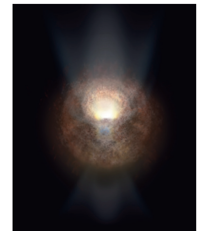
Figure 1.12: Illustration of a black hole illuminating the surrounding dense gas (Artist: Akihiro Ikeshita)
