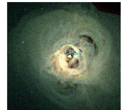
Figure 1.5: Center of Perseus galaxy cluster (NASA/CXC/IOA/Fabian et al.)
