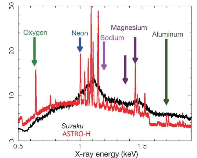
Figure 1.11: X-ray spectra from the Perseus cluster. Suzaku data is from a real observation. ASTRO-H data is a simulation and allows us to detect emission lines from rare elements, such as sodium, aluminum, and to determine abundances accurately.
