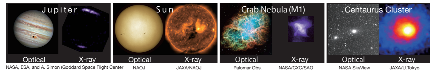
Figure 1.3: Size comparison of various sources (above), and their images in optical light and X-ray.
