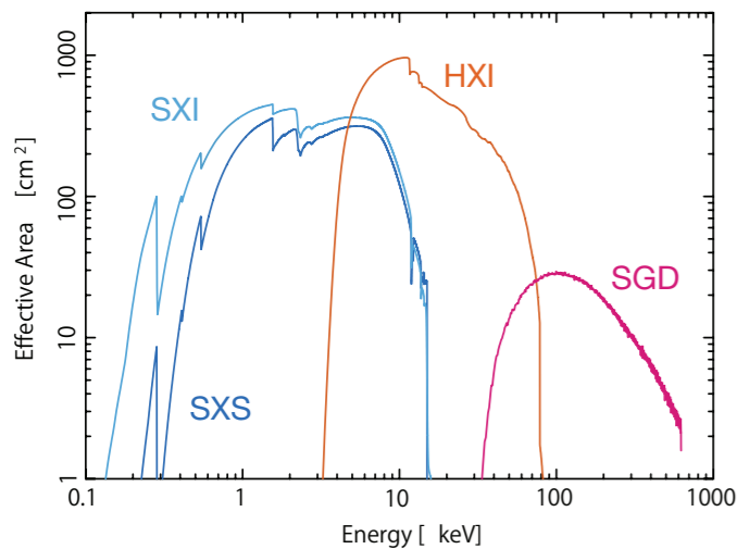
Figure 3.3: Effective area of ASTRO-H science instruments. The HXI and SGD plots are for two units.
