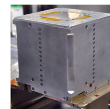
Figure 2.9: Sensor part of each semiconductor detector. In order from top: SXI, HXI, and SGD.
