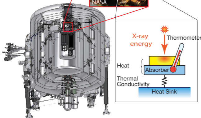
Figure 2.8: Cross-sectional diagram of SXS cooling system
