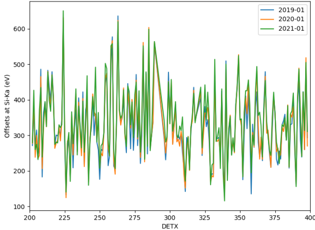
Figure C.7: Column-by-column trap depths measured from the middle Cas A pointings in 2018 (blue), 2019 (orange) and 2020 (green).
