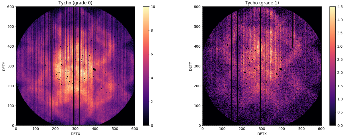
Figure C.1: Merged PC mode data of the Tycho SNR from 2014 – 2020 (exposure 2.4 Ms) showing the spatial coverage of the trap mapping observations. The left panel shows grade 0 (i.e. single pixel) events and the right panel grade 1 (i.e. vertically up-split) events. Note the reduced intensity vertical striations in some columns in grade 0, which appear as corresponding enhanced intensity striations in grade 1, are caused by grade migration as the deepest traps release charge into trailing pixels when the CCD is clocked out in the parallel direction.
