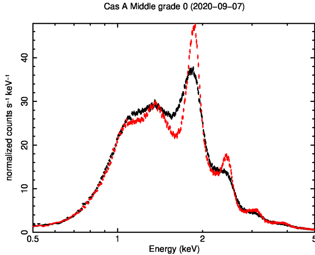
Figure C.8: Comparison of the observed and trap-corrected WT grade 0 spectra of the SNR Cas A taken in 2020-September, showing the improvements obtained when trap corrections are applied. The FWHM of the Si-K \alpha line is 293 \pm 34 eV for the uncorrected spectrum and 194 \pm 25 eV for the trap-corrected spectrum.
