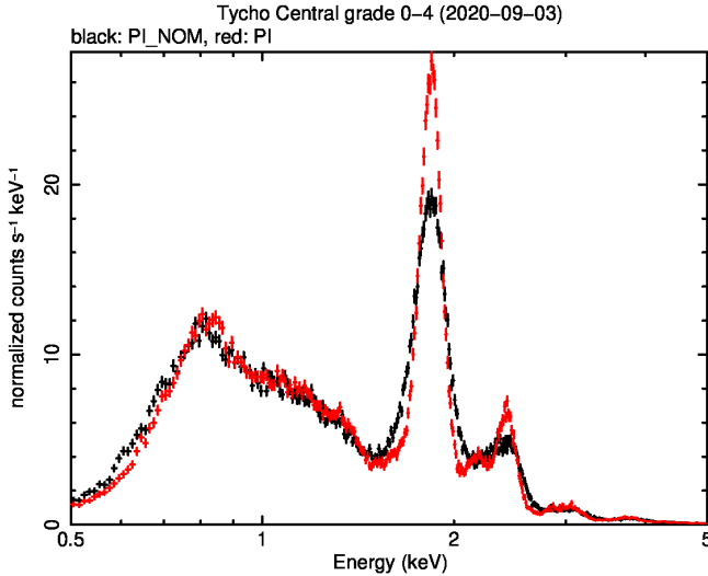
Figure C.5: Comparison of the observed and trap-corrected PC grade 0 – 4 spectra of the Tycho SNR taken in 2020-September, showing the improvements obtained when trap corrections are applied. The FWHM of the Si-K \alpha line is 234 \pm 24 eV for the uncorrected spectrum and 160 \pm 10 eV for the trap-corrected spectrum.
