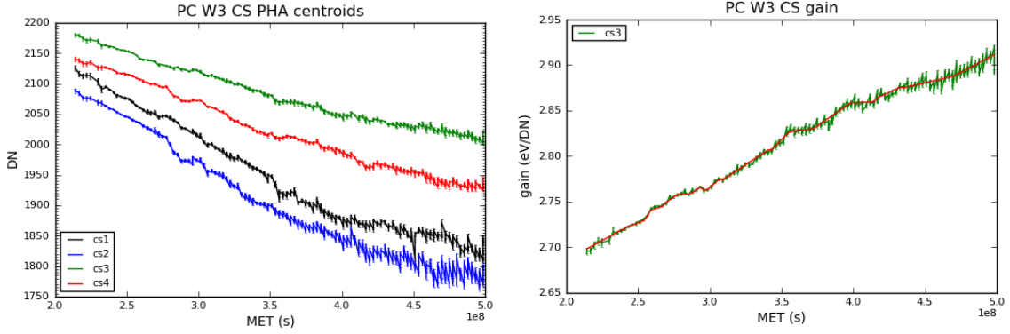
Figure 3: Swift -XRT CCD measurements from the corner source data at a CCD temperature of -60^\circ\text{C} from 2007-Sep-05 to 2016-Nov-01. The left panel shows the measured ^{55}\text{Fe} line centroids from the four corner sources. The right panel shows the gain coefficient (GC0_TRAP) estimated using equation A.11 and used for trap-corrected spectra (in green the measured monthly averaged gain values, in red the modelled gain evolution with time). Error bars are 1\sigma estimates.
