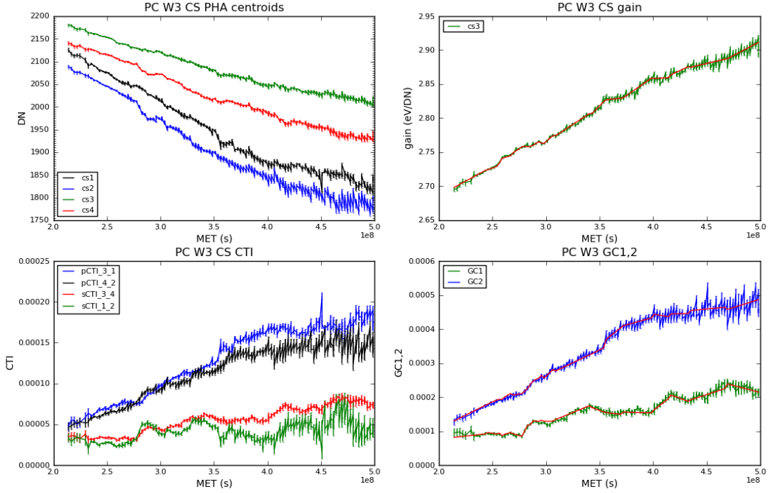
Figure B.2: Swift -XRT CCD gain and CTI measurements from the corner source data at a CCD temperature of -60^{\circ}\text{C} from 2007-Sep-05 to 2016-Nov-01. No trap-correction has been applied to the data. The top-left panel shows the measured ^{55}\text{Fe} line centroids. The top-right panel shows the gain coefficient ( GC0 ) estimated using equation A.11. The bottom-left panel shows the measured CTI coefficients for the 4 pairs of corner sources. The bottom-right panel shows the estimated gain file GC1 (serial) and GC2 (parallel) coefficients. (Error bars are 1\sigma estimates.)
