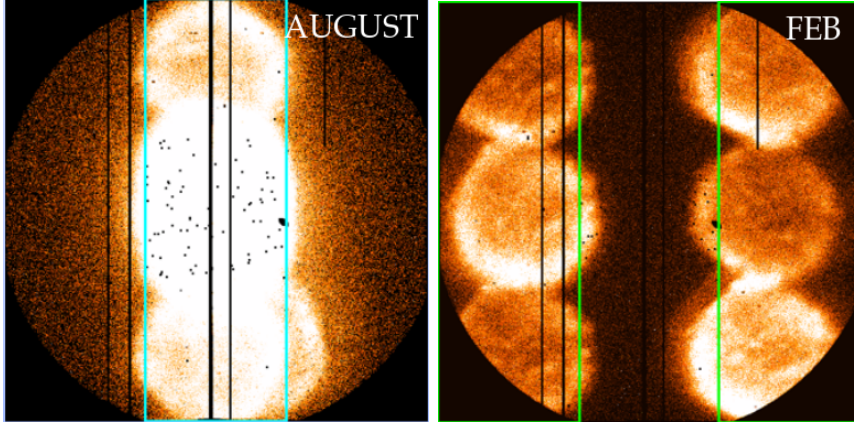
Figure 1: PC trap mapping - Previous observation strategy for the derivation of the PC mode gain files, illustrated with the observations taken during the 2014-2015 campaign. During the summer/autumn epoch the Tycho SNR was positioned to cover the central strip of the CCD ( left panel ), while during the winter/spring epoch the observations covered the left and right sides of the CCD ( right panel ).
