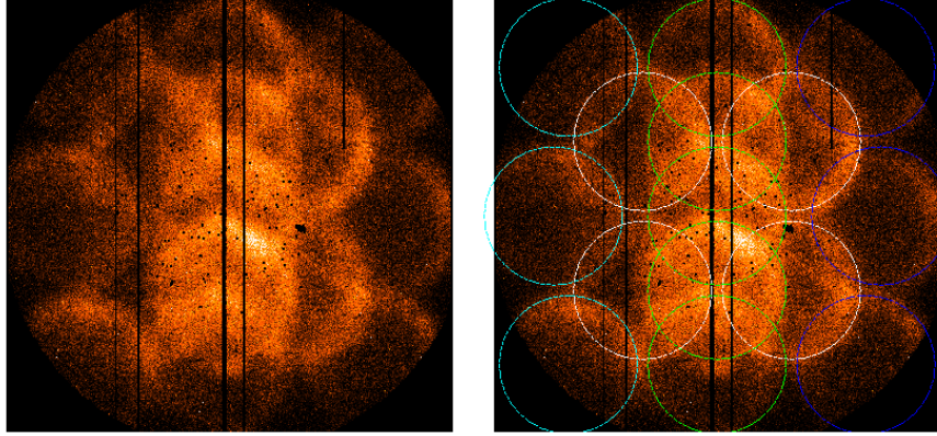
Figure 2: PC trap mapping - New observation strategy for the derivation of the new PC mode gain file swxpcgains6_20010101v016.fits , illustrated with the observations taken during the Fall 2016 campaign. The Tycho SNR was positioned to get a coverage of the CCD that is as uniform as possible ( left panel, illustrating the CCD coverage ), while still slightly prioritising the central column ( right panel, illustrating the individual pointings ).
