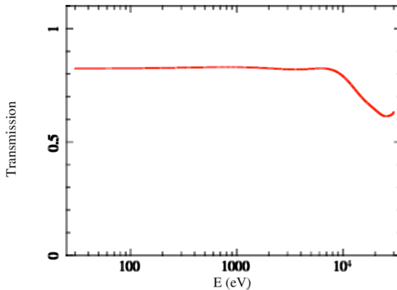
Figure 2: Transmission due to the gate valve structure as a function of energy (without the Be filter/Mesh). Neutral Density Filter
