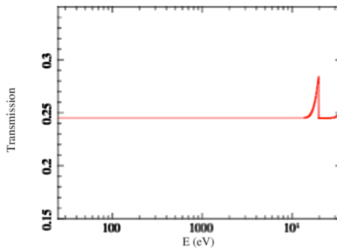
Figure 4: Transmission due to the neutral density filter as a function of energy.
