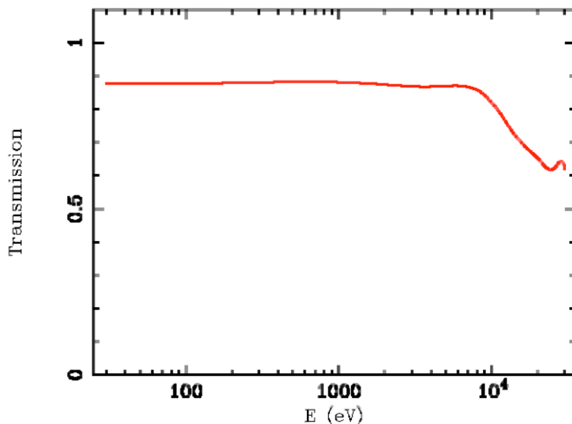
Transmission due to the gate valve structure as a function of energy (without the Be filter/Mesh).
