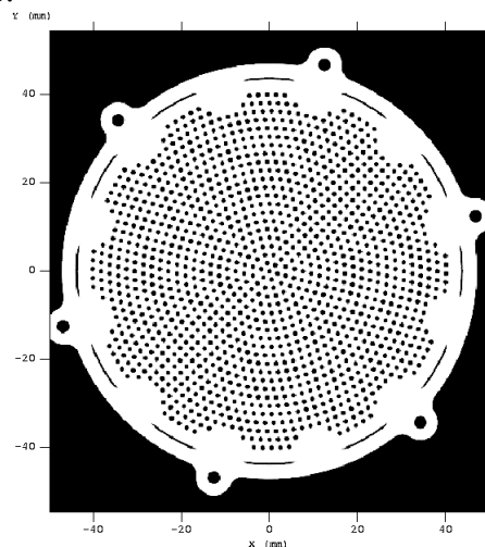
Figure 3: 2-D image in the primary extension of the neutral density filter CALDB file. White areas are pixels with full covering, black areas are partially transparent, the effective covering factor of each pixel is equal to
