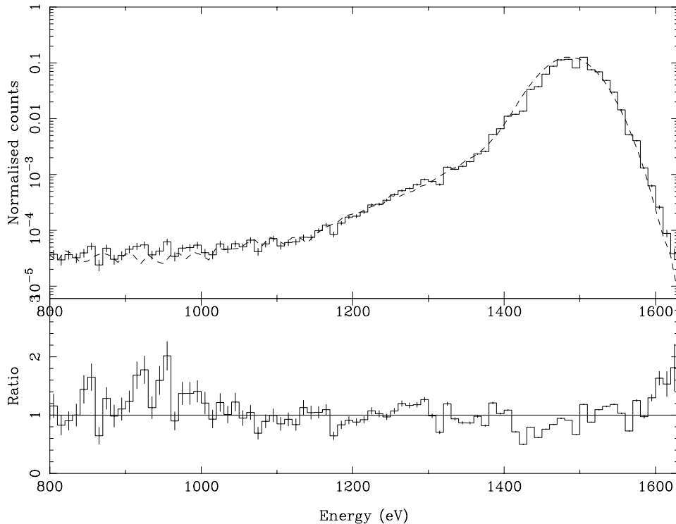
Figure 5. Spectral data from laboratory calibration (dashed line) and simulated spectrum (solid line) for Aluminium K_{\alpha} line at 1.487 keV is shown for comparison. Error bars show the statistical precision of the simulation.
