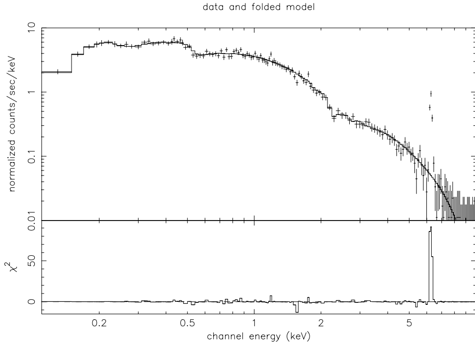
Figure 7. A simulated single pixel event XRT spectrum for Photon Counting mode. The model is the absorbed power law spectrum of GRB030329 observed around 5 hours. The data include an illustrative redshifted 6.4 keV iron line of 3 keV equivalent width (not seen in GRB030329). The detectability of the iron line is shown in the lower portion of the figure.
