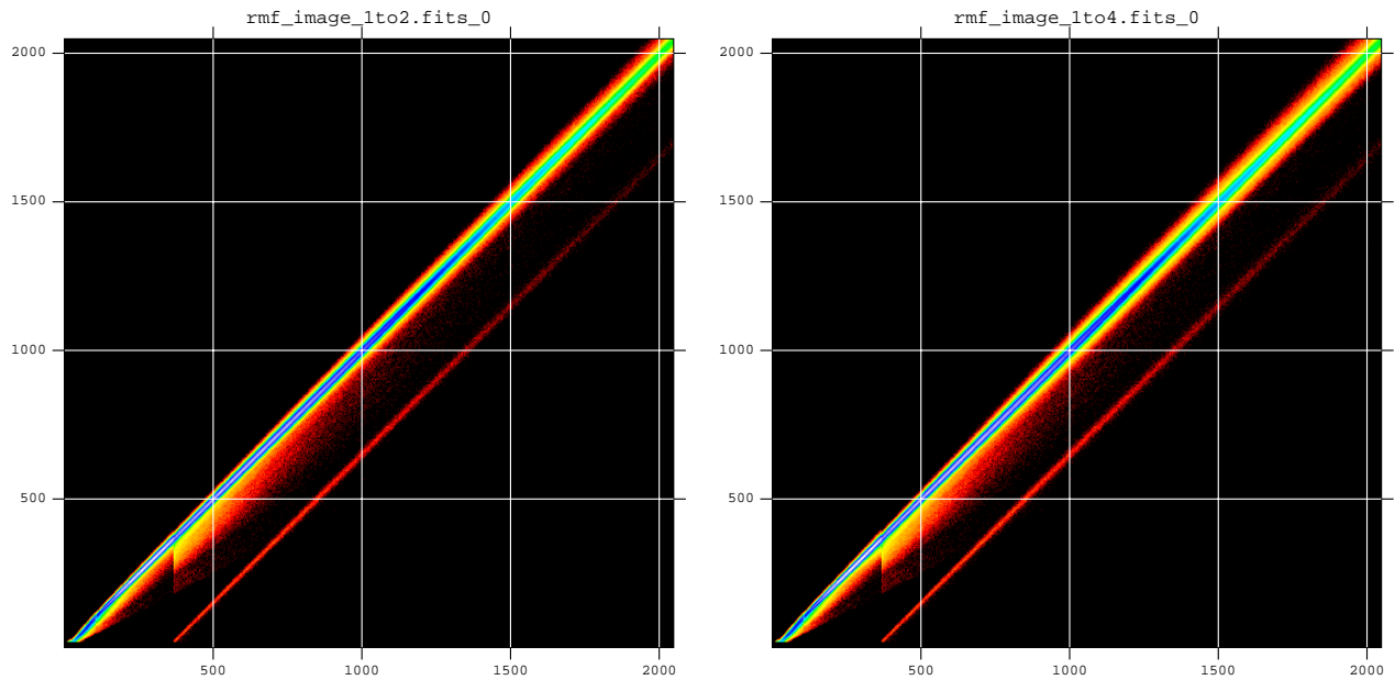
Figure 6. The CCD response for 1-2 pixel events (left) and 1-4 pixel events (right) are shown with the same linear scaling. The x-axis is the input photon energy, the y-axis the response. Both axes cover 0-10.24 keV.
