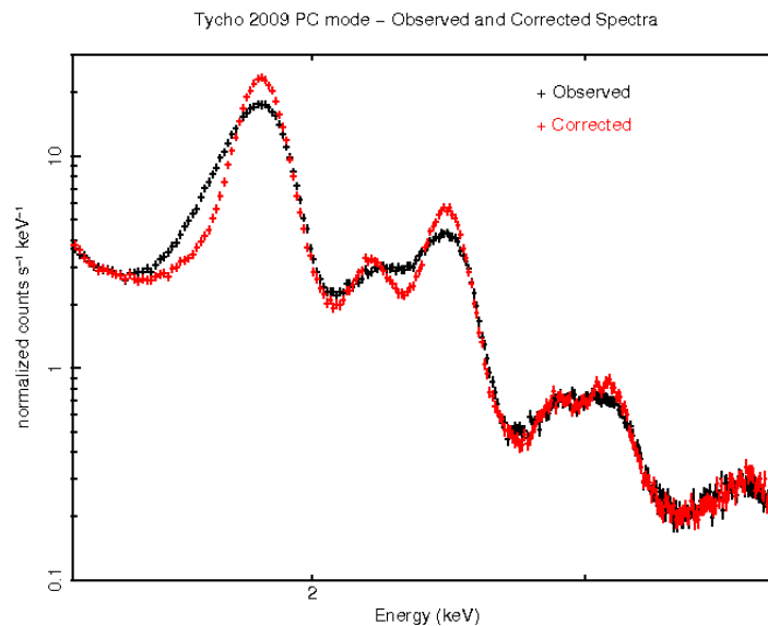
Figure C.6: Comparison of the observed and the trap corrected spectra extracted from a PC mode observation of the Tycho SNR from October 2009. The fit of the Silicon K \alpha line with an asymmetric Gaussian in IDL yielded a FWHM of 179 \pm 8 eV for the observed spectrum and of 132 \pm 3 eV for the corrected spectrum.
