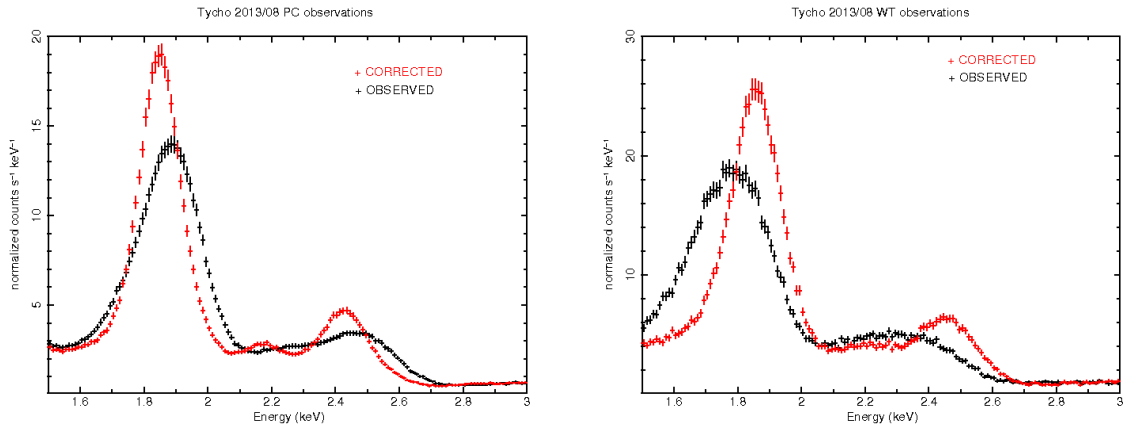
Figure 3: Comparison of non trap corrected spectra (in black) and trap corrected spectra (in red) in 2013 Tycho observations taken in PC mode (left panel) and WT mode (right panel). The resolution is higher in trap corrected PC spectra as the trap mapping analysis allows the identification and the correction of traps in individual pixels, while for WT observations with limited spatial information the trap corrections are averaged and applied over entire columns.
