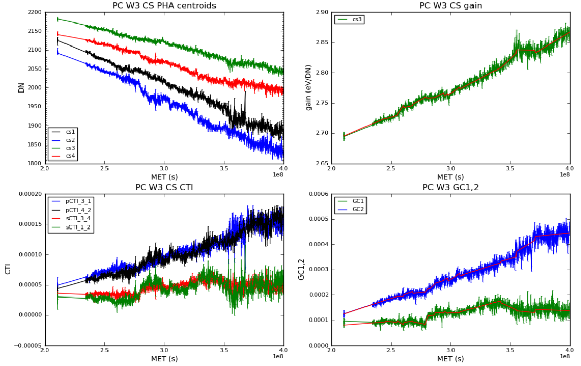
Figure B.2: Swift -XRT CCD gain and CTI measurements from the corner source data at a CCD temperature of -60^{\circ}\text{C} from 2007-Sep-05 to 2013-Sept-30. No trap-correction has been applied to the data. The top-left panel shows the measured ^{55}\text{Fe} line centroids. The top-right panel shows the gain coefficient ( GC0 ) estimated using equation A.11. The bottom-left panel shows the measured CTI coefficients for the 4 pairs of corner sources. The bottom-right panel shows the estimated gain file GC1 (serial) and GC2 (parallel) coefficients. (Error bars are 1\sigma estimates.)
