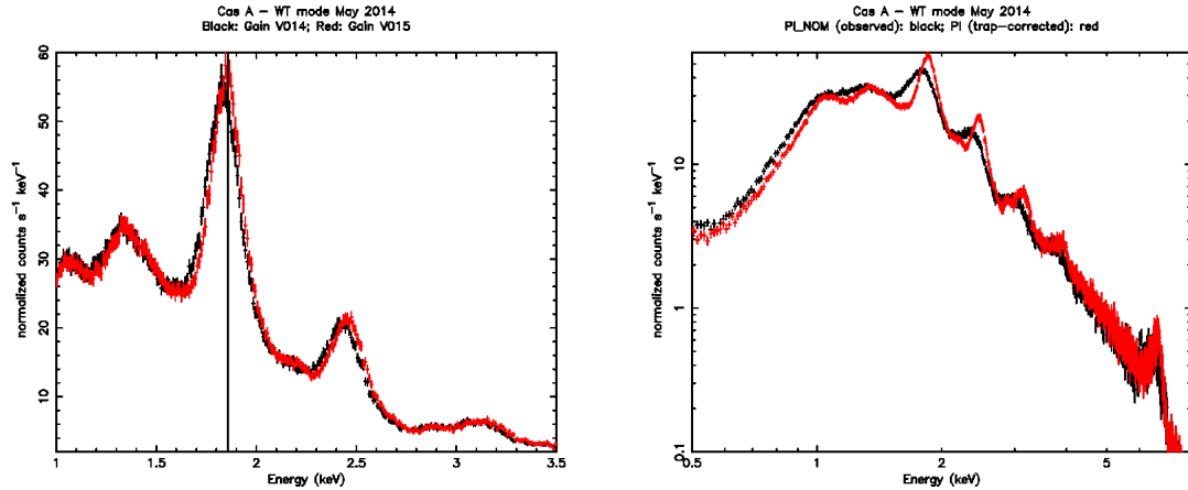
Figure 1: Cas A observations in WT mode from May 2014. Left panel - The spectrum extracted using the current CALDB WT gain file (v014), in black, is shifted to lower energies due to the effects of charge traps generated by radiation; the correct energy scale is restored when the data are processed with the new WT gain file (v015), in red, included in this release. The vertical black line is at the Silicon reference energy of 1.863 KeV. Right panel - Comparison of the observed spectrum, in black, and the trap-corrected spectrum, in red, when the data are processed with the new WT gain file (v015).
