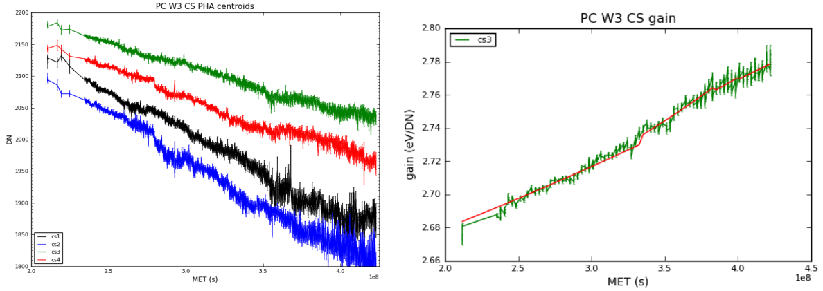
Figure 2: Swift -XRT CCD measurements from the corner source data at a CCD temperature of -60^{\circ}\text{C} from 2007-Sep-05 to 2014-May-30. The left panel shows the measured ^{55}\text{Fe} line centroids from the four corner sources. The right panel shows the gain coefficient (GC0_TRAP) estimated using equation A.11 and used for trap-corrected spectra (in green the measured monthly averaged gain values, in red the modelled gain evolution with time). Error bars are 1\sigma estimates.
