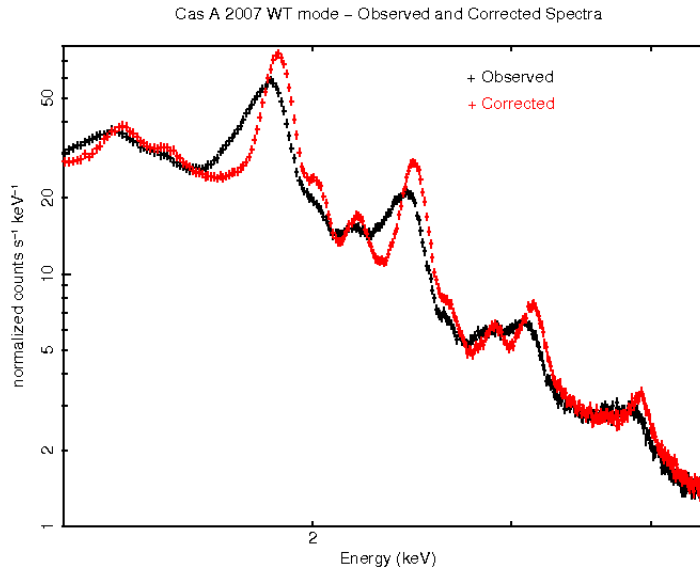
Figure C.7: Comparison of the observed and the trap corrected spectra extracted from WT observations of the Cas A SNR in October of 2007. The fit of the Silicon K\alpha line with an asymmetric Gaussian in IDL yielded a FWHM of 152 \pm 13 eV for the observed spectrum and of 106 \pm 3 eV for the corrected spectrum.
