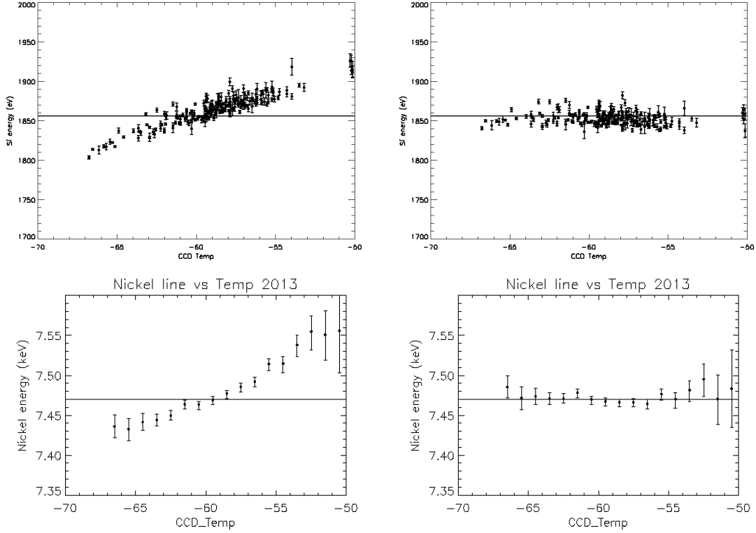
Figure 5: The temperature dependence of the trap losses is seen in the Tycho observations and in the PC datasets used to extract the instrumental Nickel K\alpha line (left panels). Processing the PC data with the updated gain file, that includes temperature dependent trap tables, the Silicon line in Tycho and the instrumental Nickel are close to the expected value at all temperatures.
