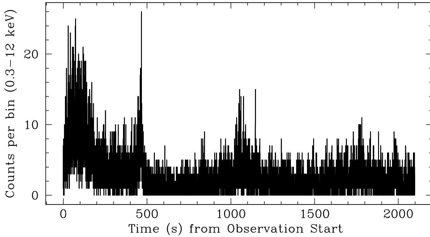
NICER: GX_339-4 Light Curve in 0.1 s bins
