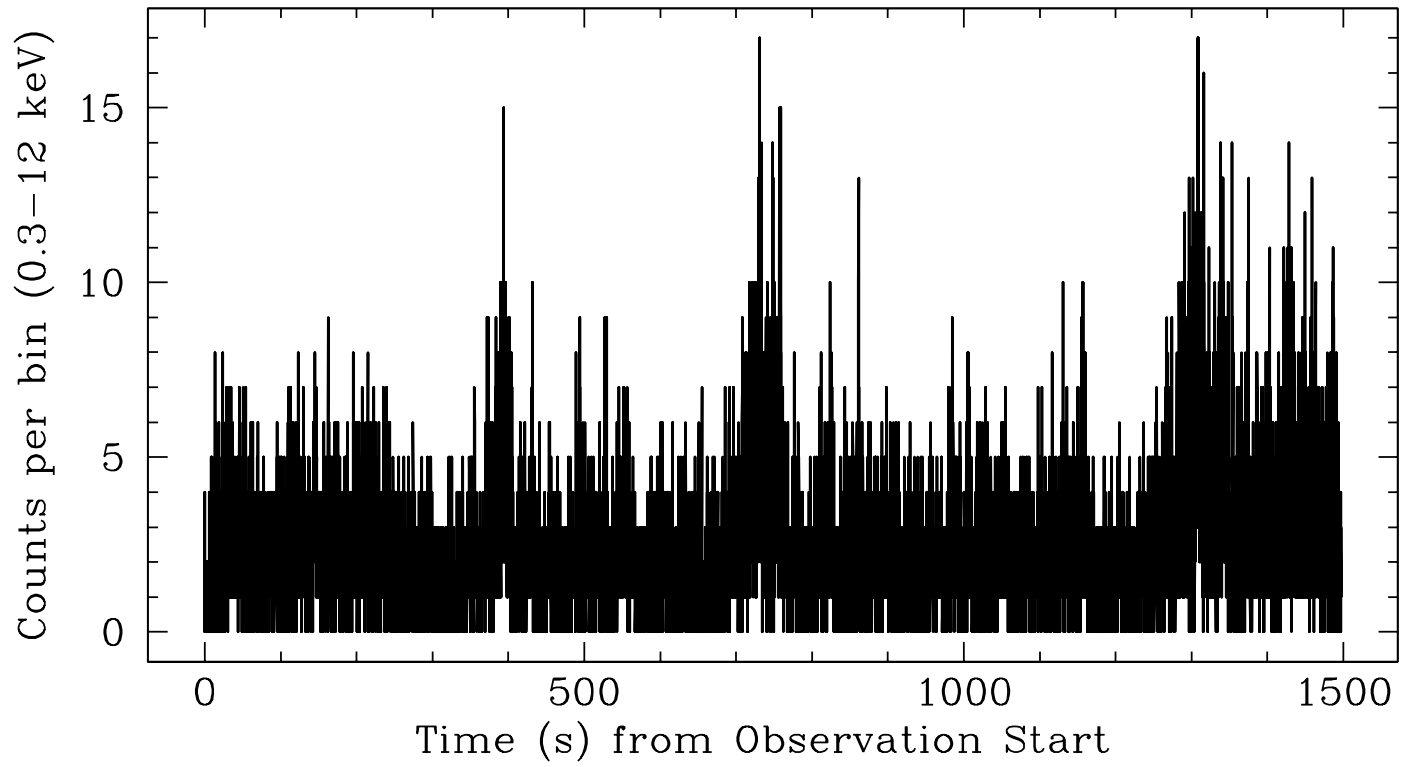
NICER: GX_339-4 Light Curve in 0.1 s bins
