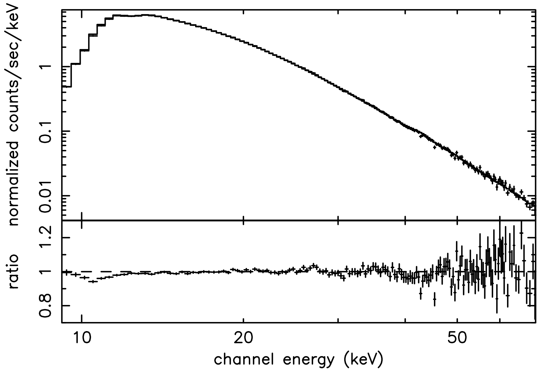
Crab XIS-nominal (20060814)
