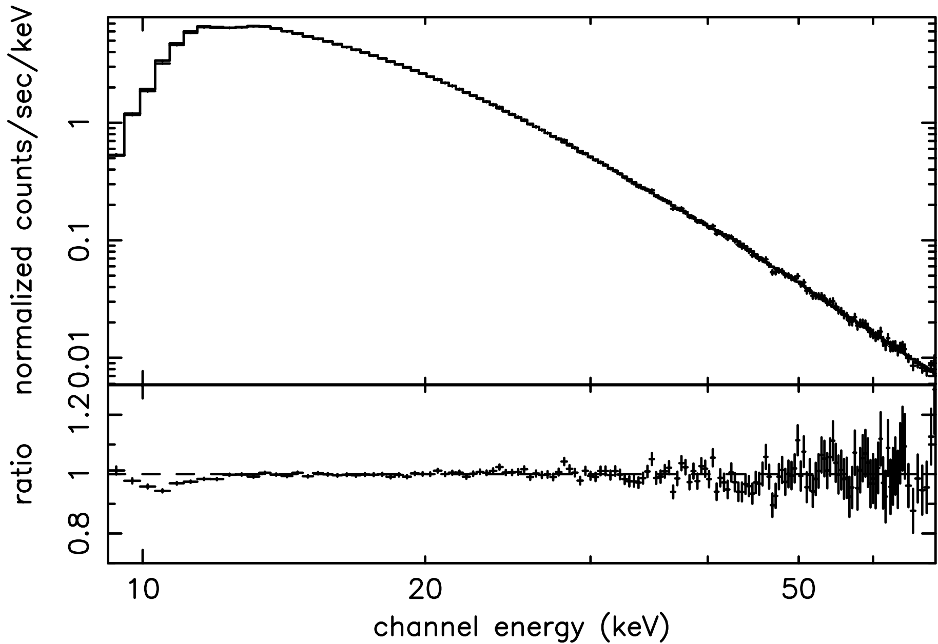
Crab HXD—nominal (20060814)
