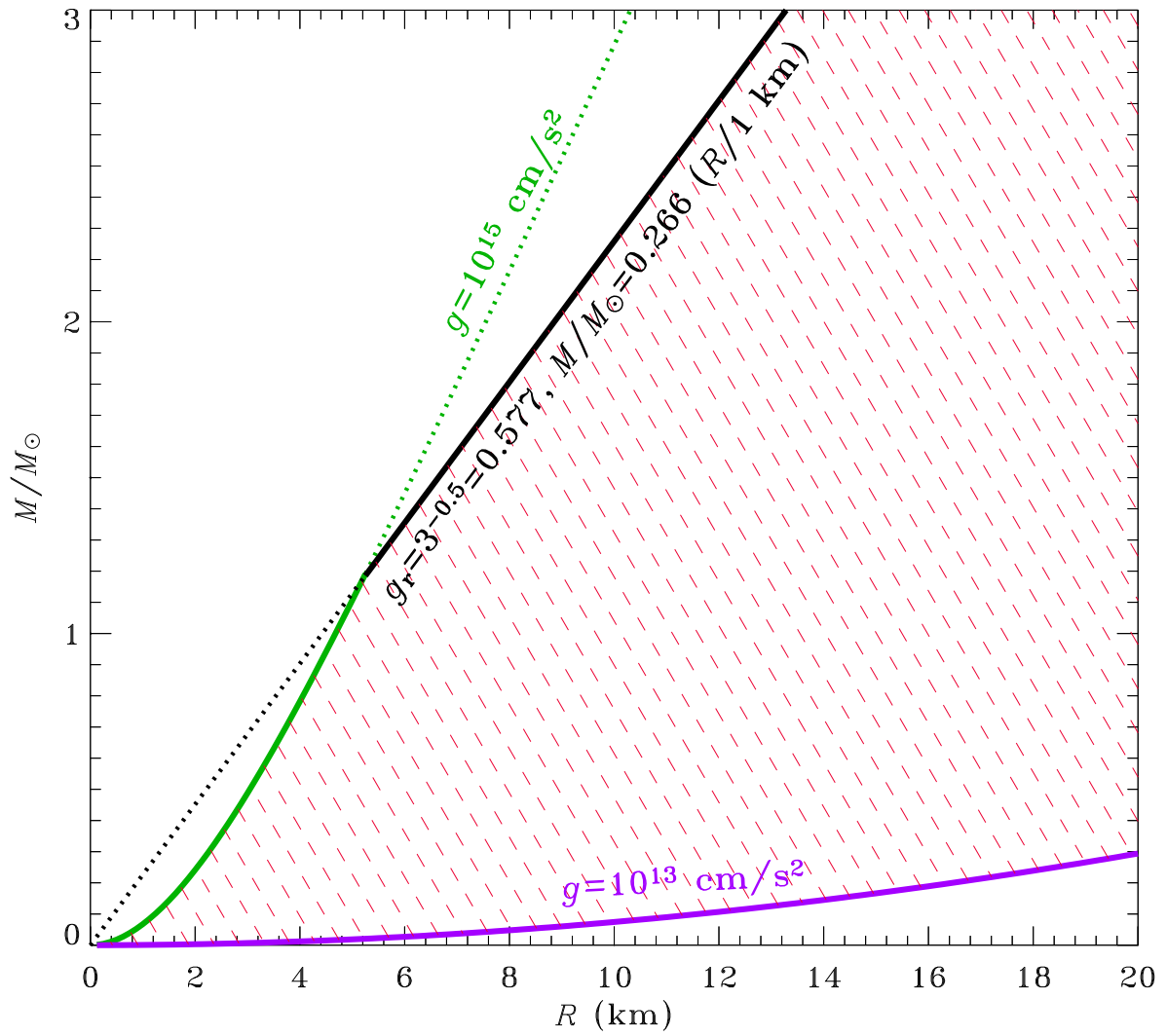
Allowed M-R domain in the NSAGRAV model of XSPEC
